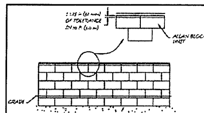
Figure 13: Vertical Control
