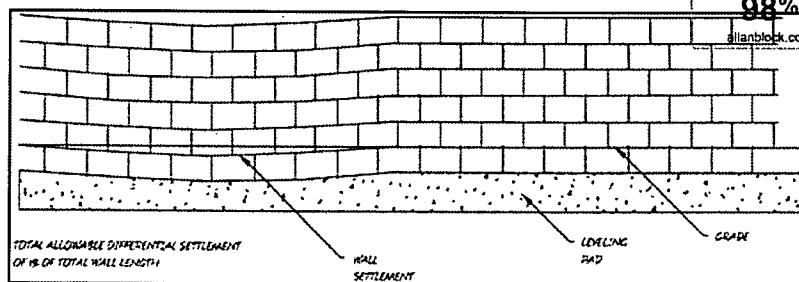
Figure 14: Differential Settlement
