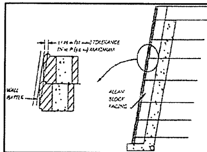
Figure 15: Horizontal Control
