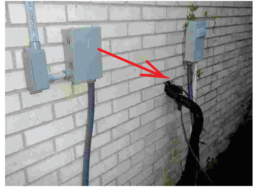
Wall penetrations are not sealed
