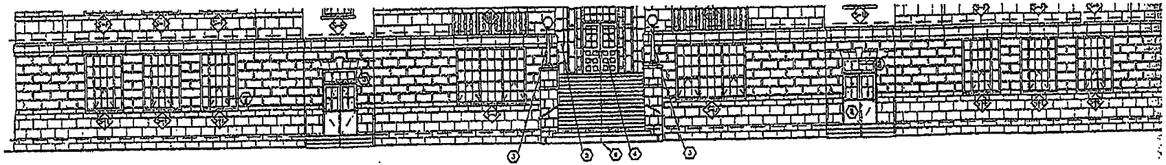
1 EAST ELEVATION
