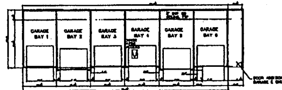
Floor Plan - Garage SCALE: 1/8" = 1'-0" GARAGES ARE LCE = LIMITED COMMON ELEMENT
