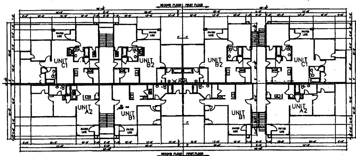
Floor Plan - Building Type I
