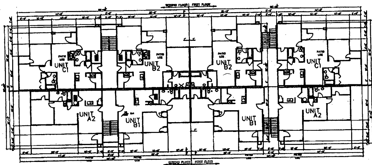
Floor Plan - Building Type I
