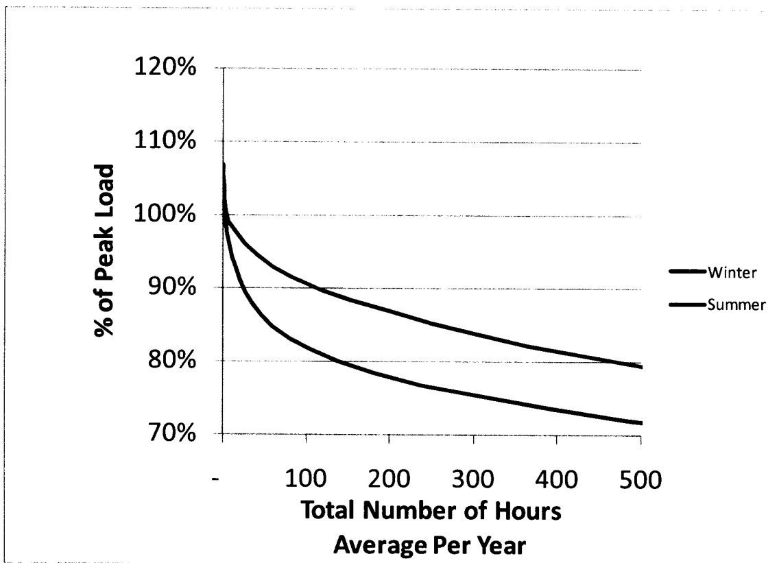
Figure 2. Frequency of High Load Hours for Winter and Summer
