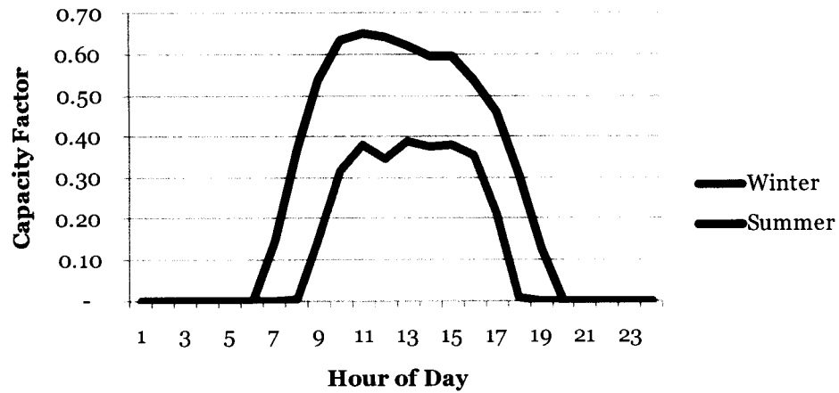
Figure 9. Solar Profile
