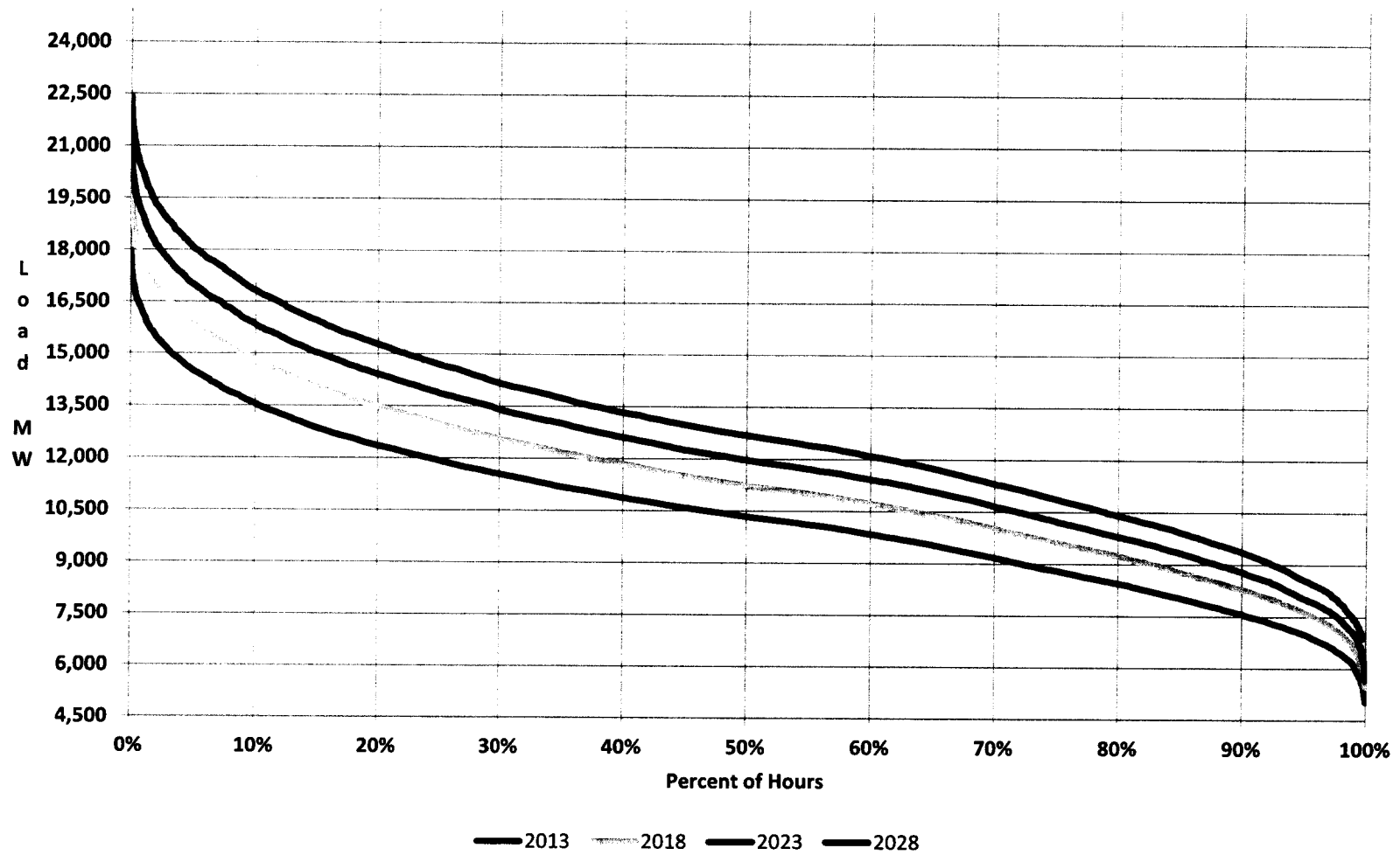
Chart C-7 Load Duration Curve with Energy Efficiency Programs
