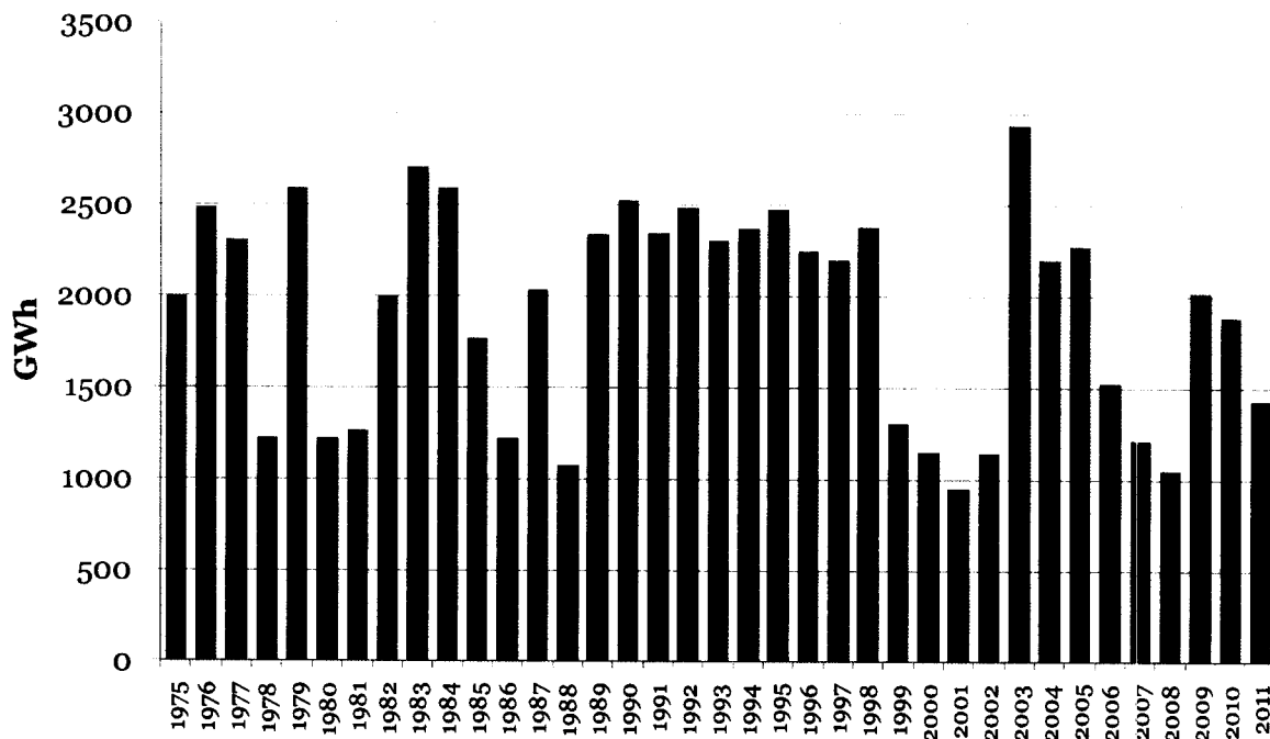
Figure 7. Hydro Energy by Weather Year
