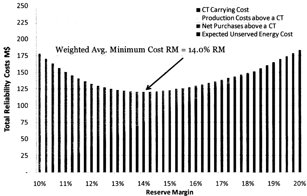
Figure 17. Base Case Weighted Average Economic Reserve Margin
