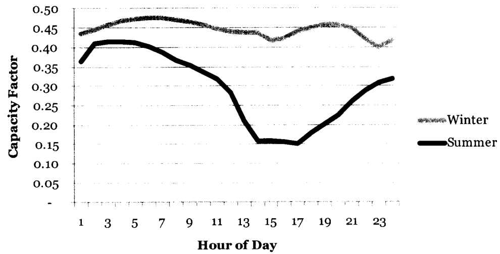
Figure 10. Wind Profile
