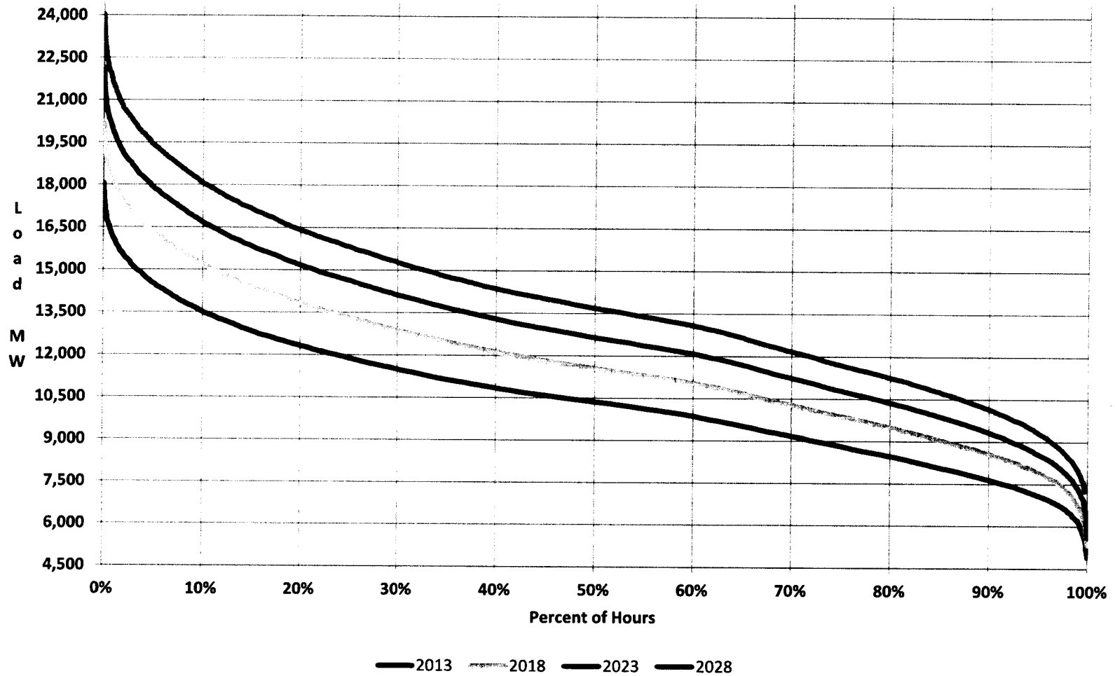
Chart C-5 Load Duration Curve without Energy Efficiency Programs
