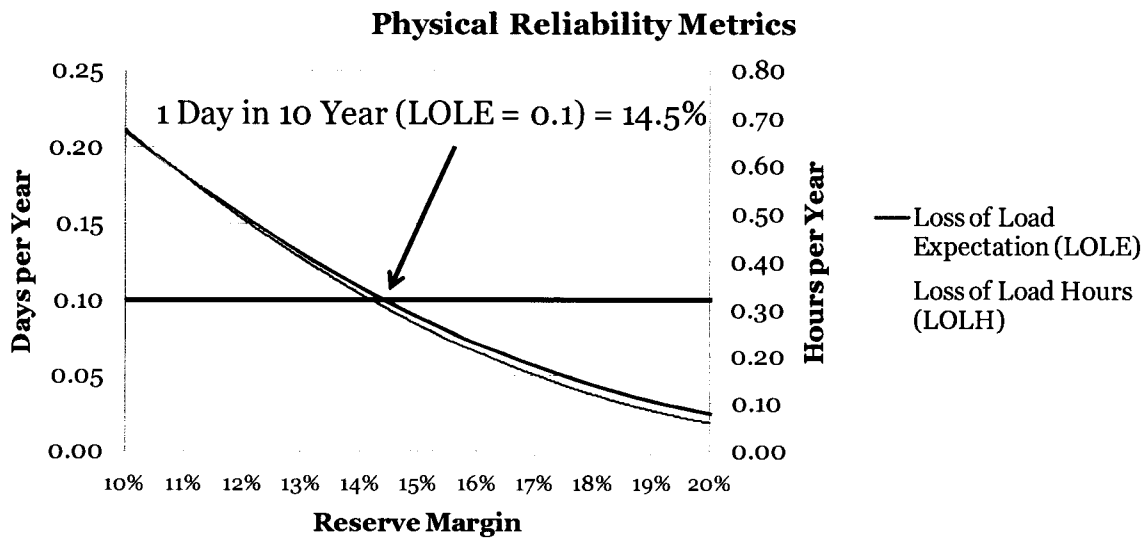
Figure 15. Base Case LOLE and LOLH
