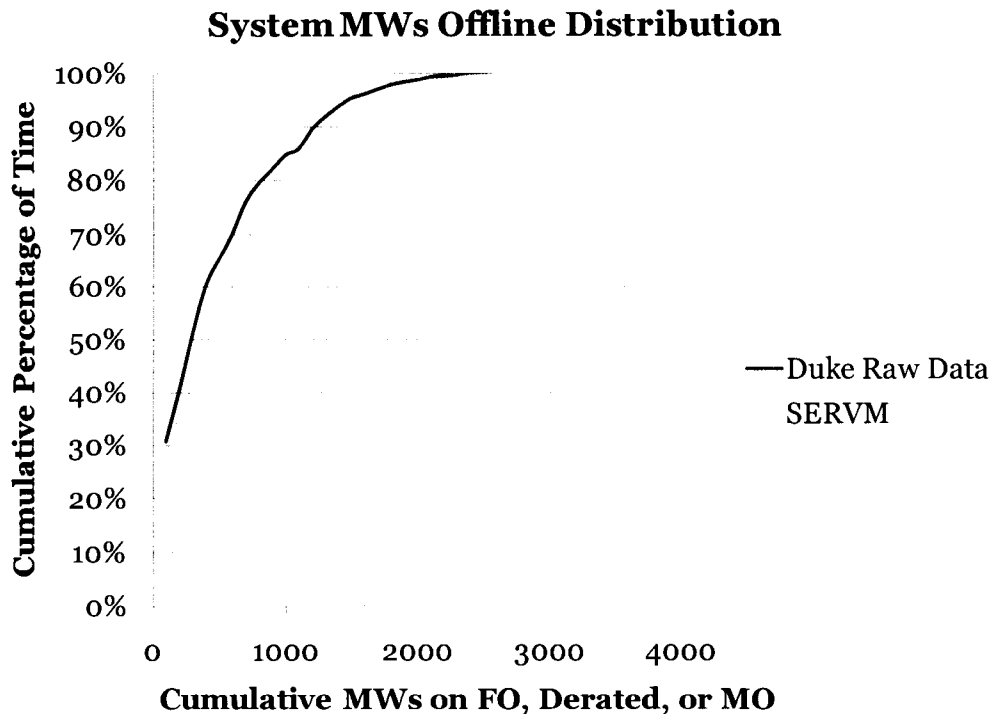
Figure 11. System Capacity Offline as a Percentage of Time
