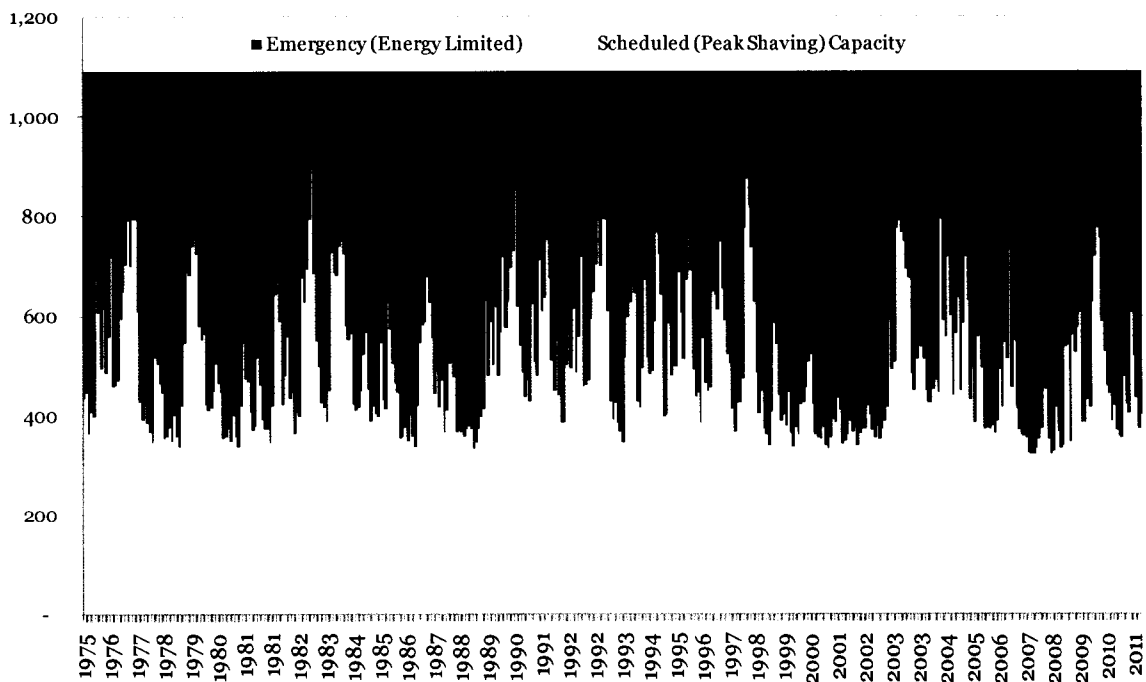
Figure 6. Scheduled Capacity versus Emergency Capacity
