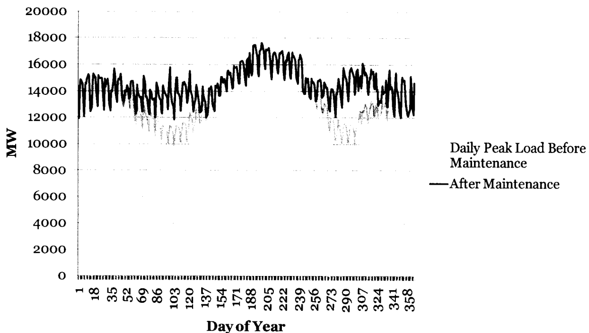
Figure 12. Daily Peak Load Plus Planned Maintenance Requirement
