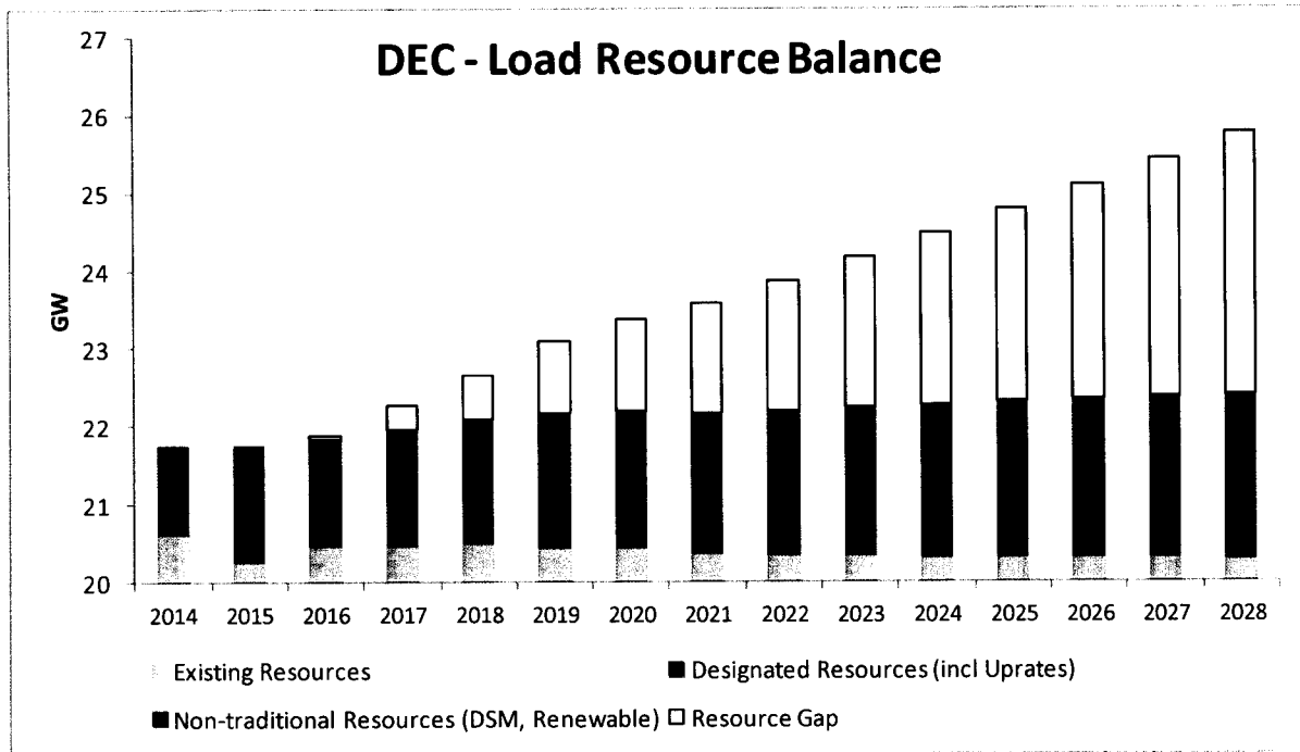
Chart 8-B DEC Load Resource Balance
