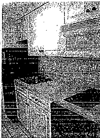
Galley Kitchen
