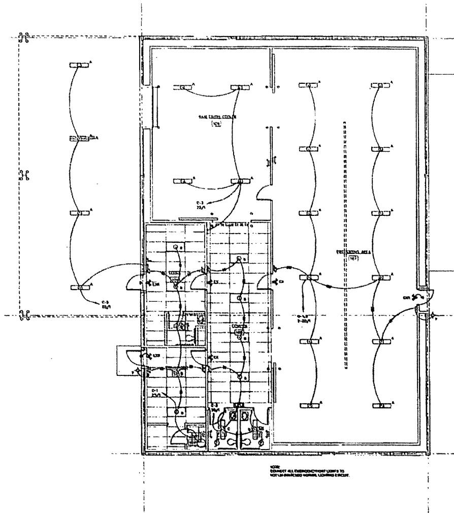
ELECTRICAL LIGHTING PLAN 3/16" = 1'-0"
