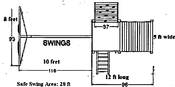
Safe Play Area: Add 10 ft on each side
