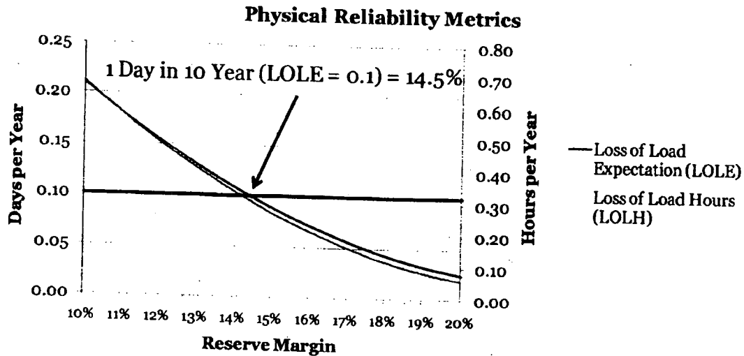
Figure ES1. Physical Reliability Metrics
