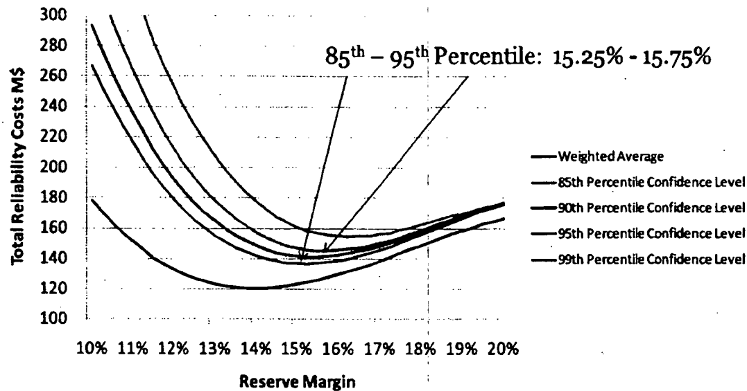
Figure 19. Risk Adjusted Reserve Margins
