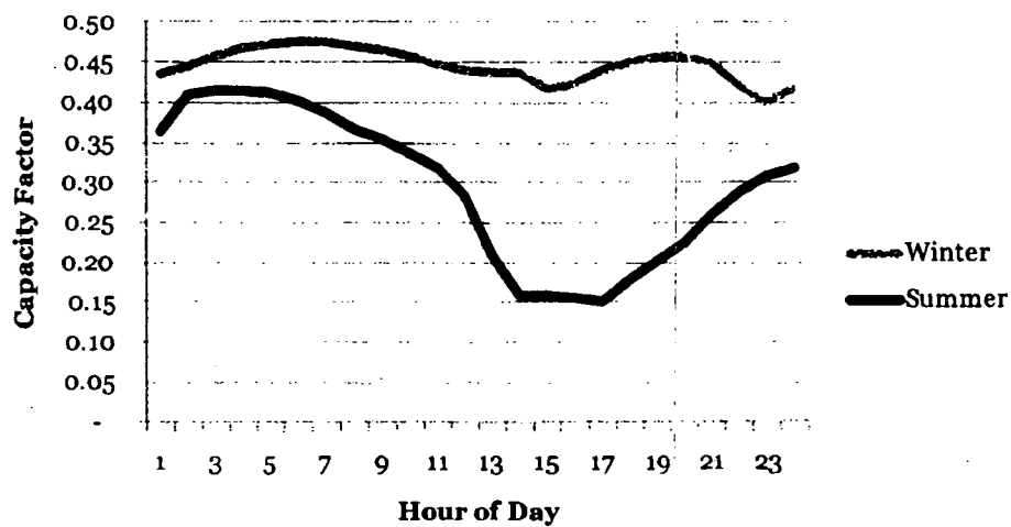
Figure 10. Wind Profile
