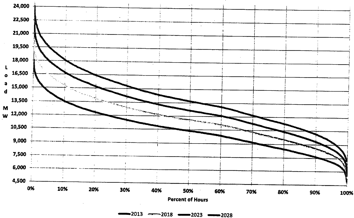
Chart C-5 Load Duration Curve without Energy Efficiency Programs
