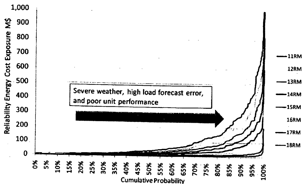
Figure ES3. Distribution of Reliability Energy Costs
