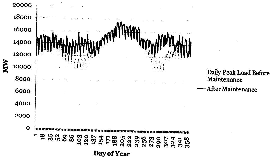
Figure 12. Daily Peak Load Plus Planned Maintenance Requirement
