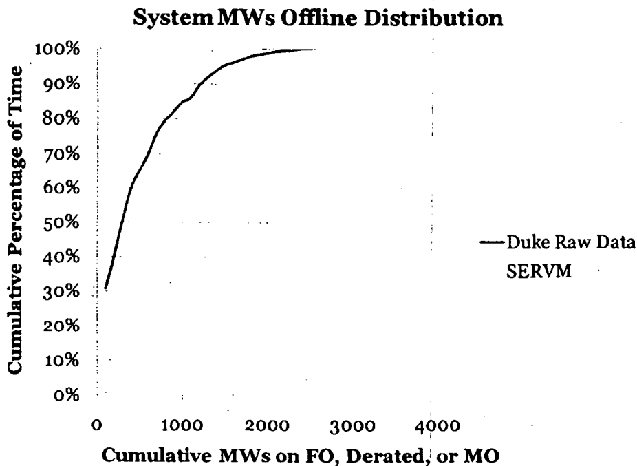
Figure 11. System Capacity Offline as a Percentage of Time
