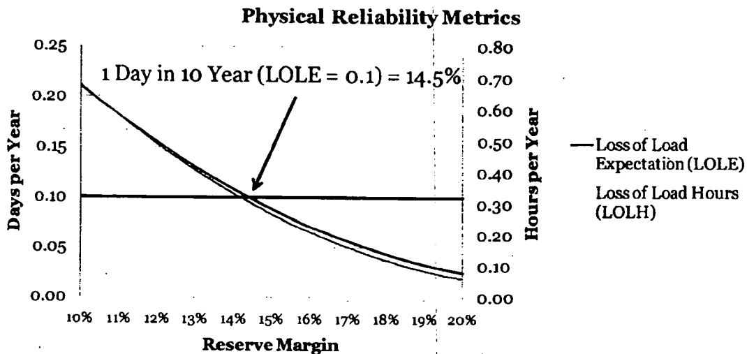
Figure 15. Base Case LOLE and LOLH
