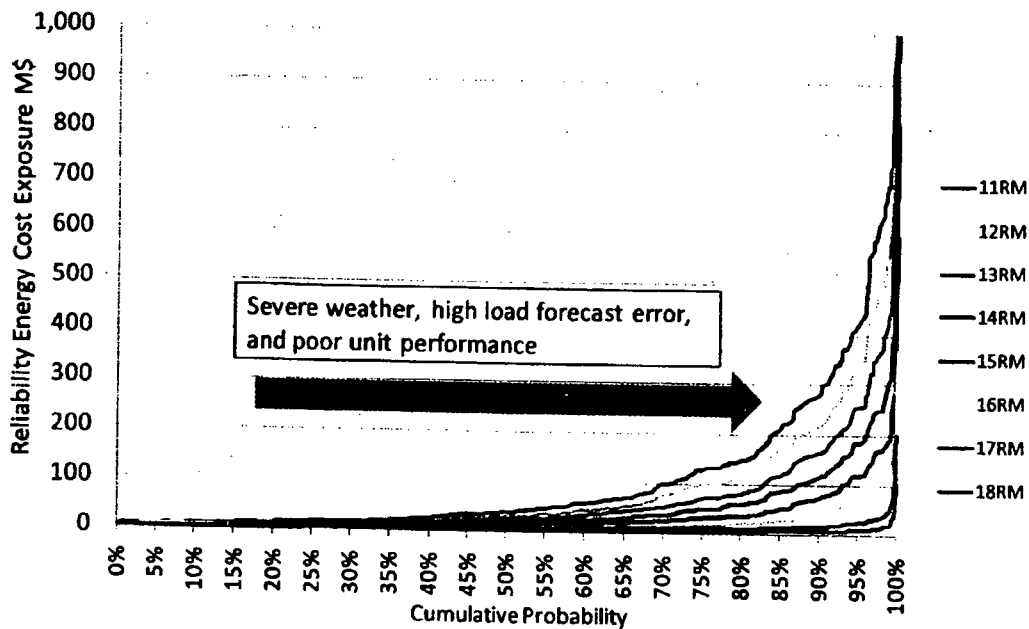
Figure 18. Base Case Reliability Cost Exposure Distribution
