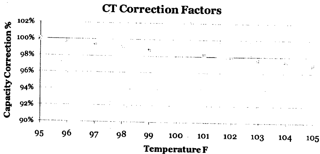
Figure 5. Summer Rating Capacity Multipliers
