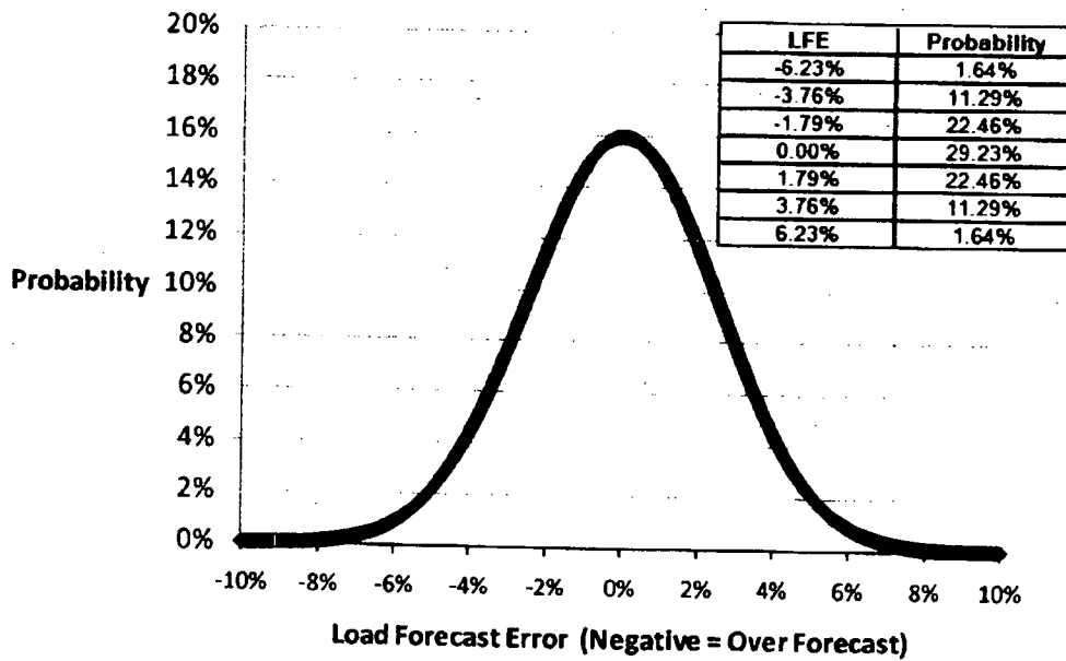
Figure 4. Load Forecast Error
