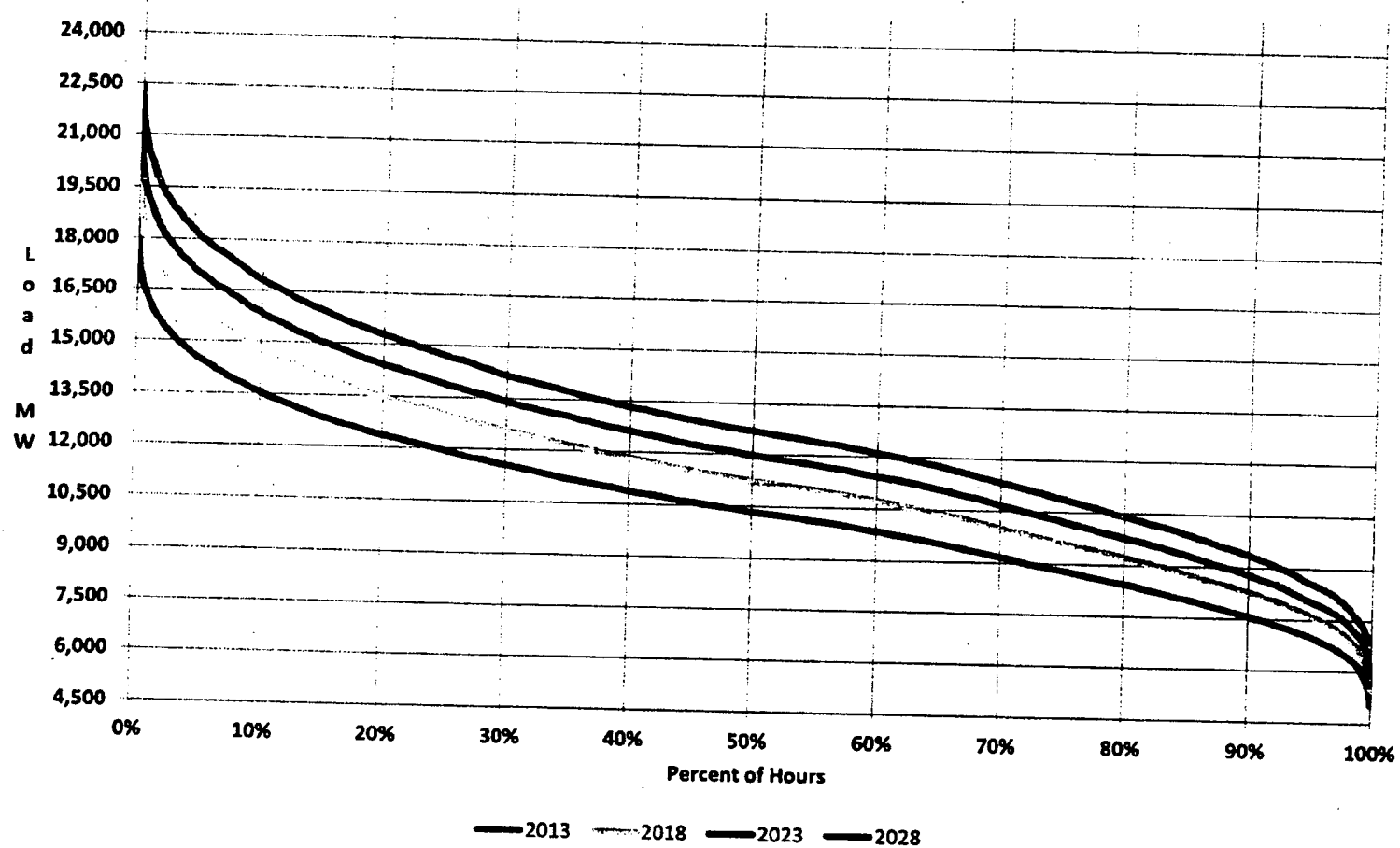
Chart C-7 Load Duration Curve with Energy Efficiency Programs
