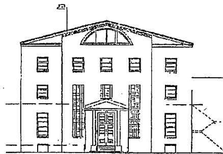
EAST ELEVATION SCALE 1/8" = 1'-0"
