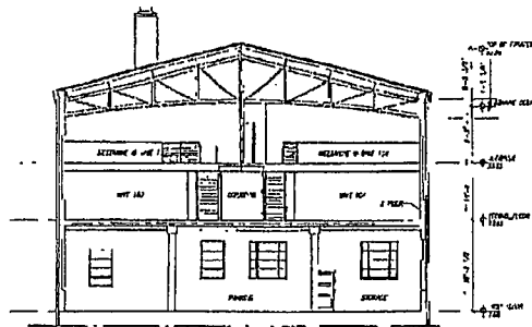
3 NORTH-SOUTH GYM SECTION SCALE 1/8" = 1'-0"
