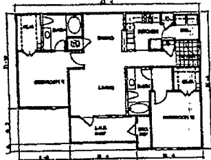
UNIT B1 - TWO BEDROOM TWO BATH
