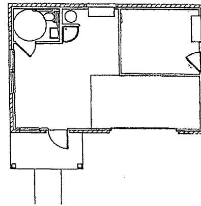
FLOOR PLAN
