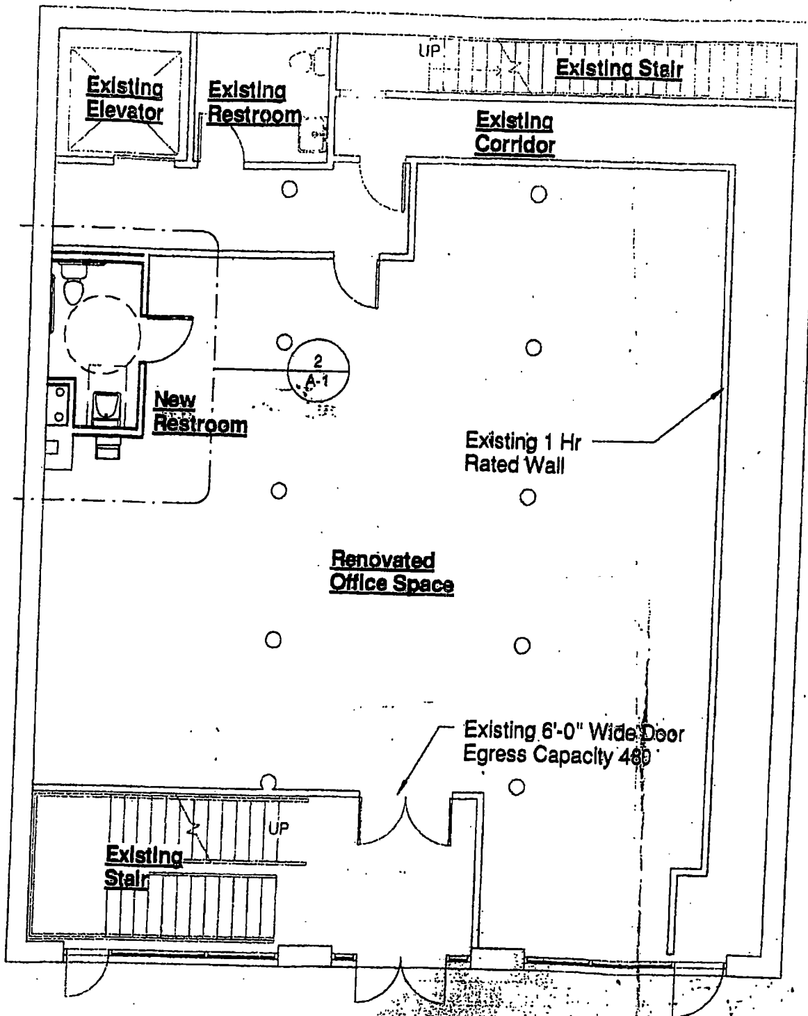
① Overall Floor Plan 1/8" = 1'-0"
